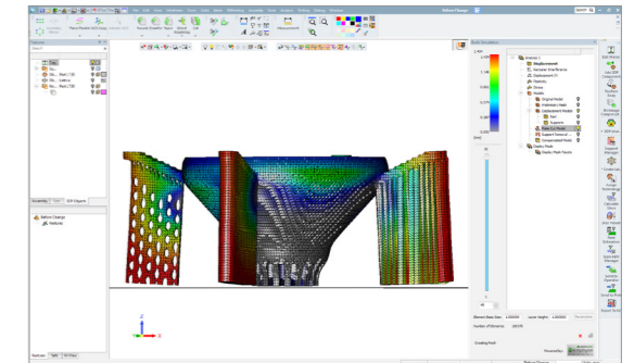
Deformation of different support types after they are cut off the plate
