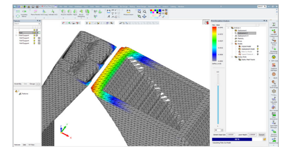
Recoater interference analysis
